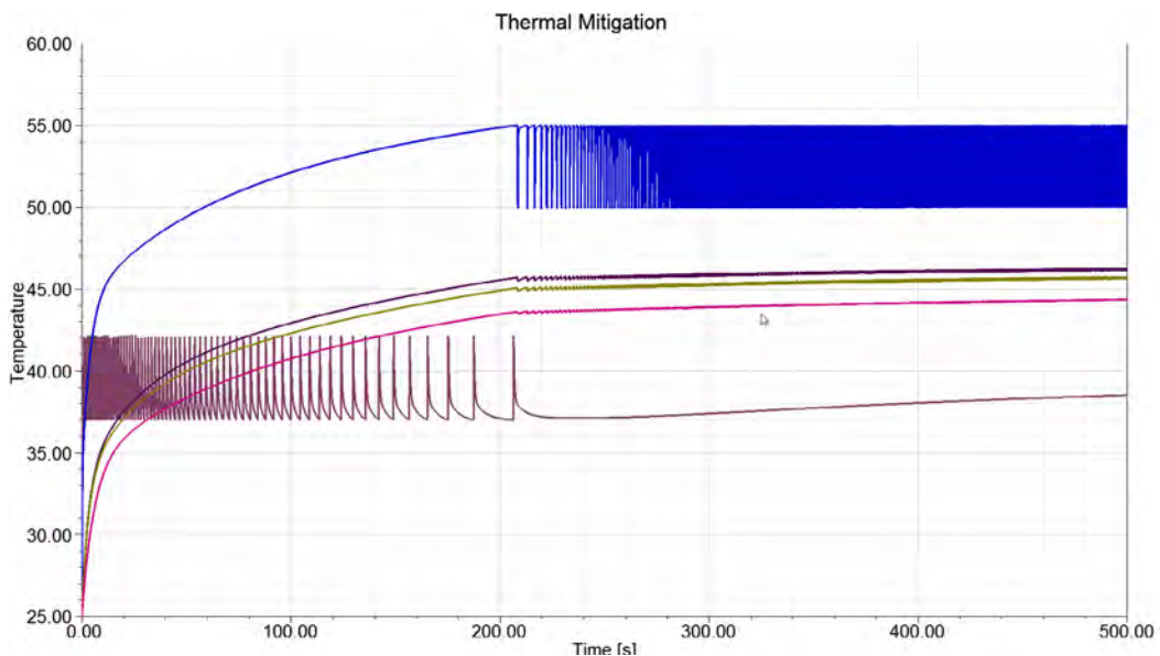
The state-space model results for model with dynamic power management
