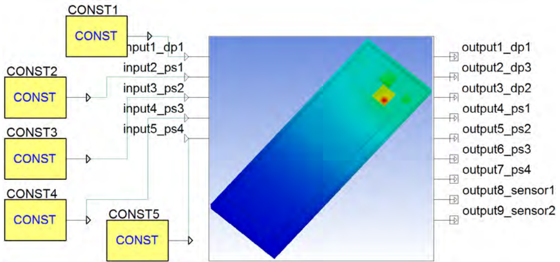
Ansys Simplorer model validation
