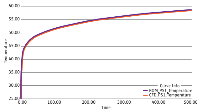
Comparison between Ansys Icepak results and the state-space model results for PS1
