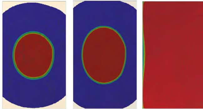
Results of contact analysis simulation with red areas indicating sufficient contact pressure to enable thermal conduction with design parameters of (left) 200 \mu\text{m} warpage, 100 \mu\text{m} TIM thickness and 800 N bolt force; (center) 60 \mu\text{m} warpage, 500 \mu\text{m} TIM thickness and 800 N bolt force; and (right) 60 \mu\text{m} warpage, 500 \mu\text{m} TIM thickness and 1200 N bolt force
