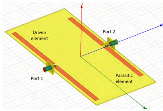
Ansys HFSS model of antenna design
