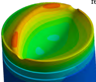
Hot spots predicted by advanced thermal modeling on the crown of the piston are addressed by changing the combustion parameters and bowl shape.
