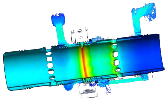
Conjugate heat transfer simulation results for the cylinder show high temperatures at the injector plane in the center of the cylinder axis.
