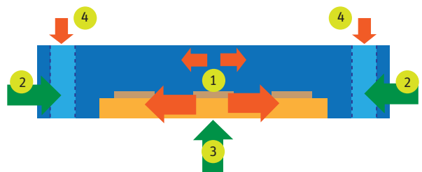
Forces during the reverse battery test: 1) expansion of substrate, 2) reaction forces exerted by bolts, 3) reaction to bolt preload and 4) bolt forces
