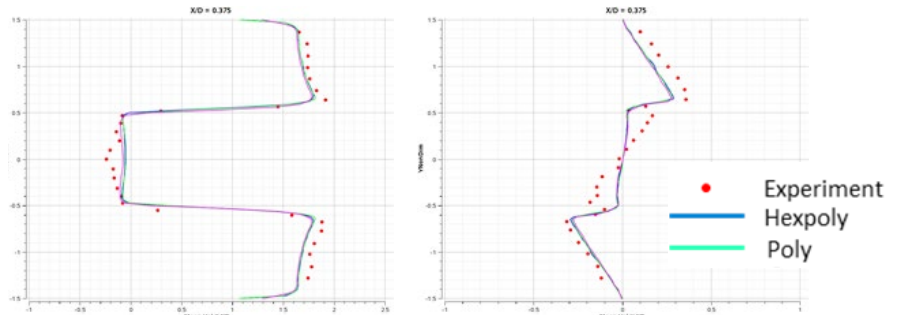
Mean X velocity (left) and mean Y velocity (right) for all polyhedral and Poly-Hexcore simulations versus physical experiments
