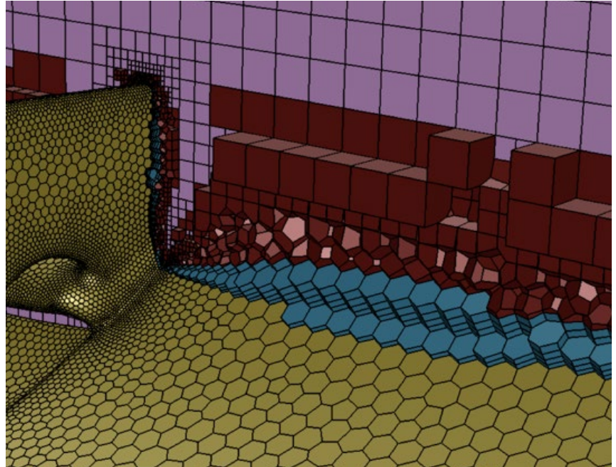
Mosaic meshing technology conformally connects hexahedral elements in the bulk region and isotropic elements in the boundary layer with polyhedral elements.
