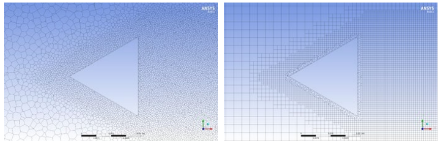
All polyhedral mesh (left) and Poly-Hexcore mesh (right)
