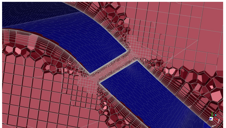
Mosaic technology creates high-quality mesh even in the submillimeter through-holes of this turbine blade.
