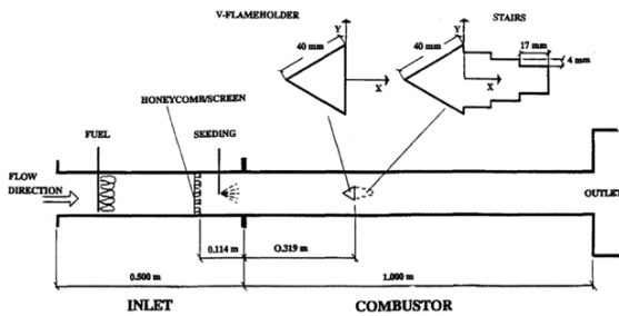
Bluff body flame holder
