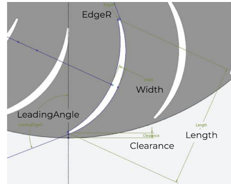
Figure 2. Simulation model of a wind turbine.
