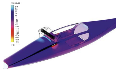
Figure 3. Unsteady-flow simulation of a wind-turbine boat hull.
