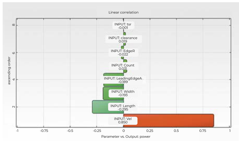
Figure 5. Effect of parameters on the wind turbine power.
