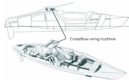
Figure 1. Structural design of the AKROS rowing boat.
