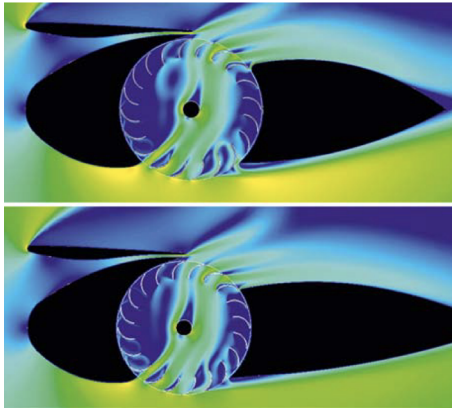
Figure 6. 2D simulation of various turbine rotor and wing geometries.
