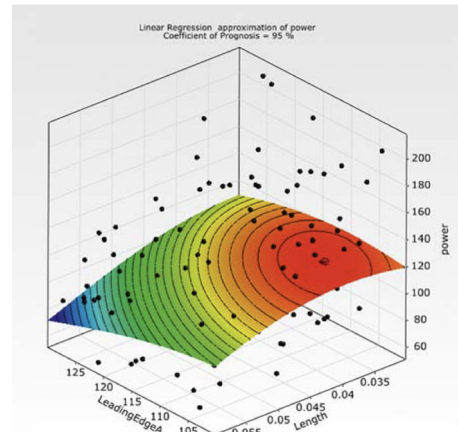
Figure 7. Response surface.
