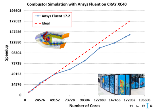
Figure 8: This image is from a benchmark [3] being run in collaboration with the High Performance Computing Center (HLRS) of the University of Stuttgart and Cray Inc. had set a supercomputing world record by scaling Ansys® Fluent® to over 172,000 computer cores on the HLRS supercomputer Hazel Hen, a Cray® XC40™ system.
