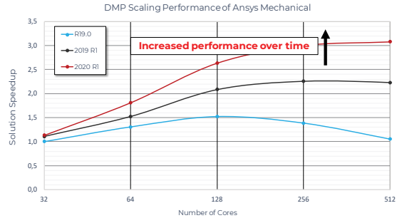
Figure 7: Release-after-release improvements made in terms of solution speedup for 9.7 million degrees of freedom model in Ansys Mechanical.
