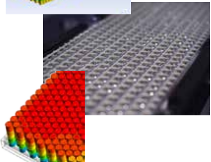
▲ Engineers modeled the transient thermal performance of the battery using ANSYS Fluent and ANSYS Simplorer over a lap of the Nürburgring Grand Prix race track.
