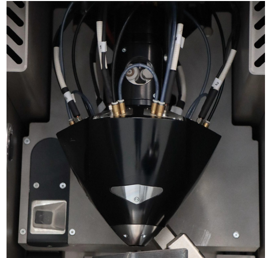
Figure 1. Meltio Technology - Printhead inside of Meltio M450.
