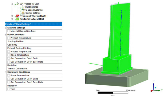
Figure 3. G-code weld path displayed on the turbine blade and process parameters used in Ansys 2023 R2.
