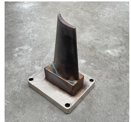
Figure 8. Turbine blade printed (DED) on the base.
