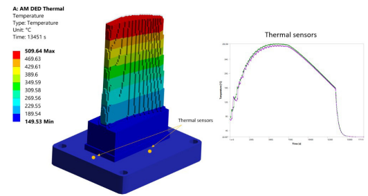
Figure 4. Overheating in the upper layers and thermal sensors captured with the simulation.
