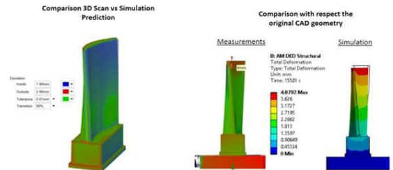
Figure 5. (a) Comparison between the 3D scan versus the simulation prediction; (b) comparison between the measurements, simulation results, and nominal geometry.
