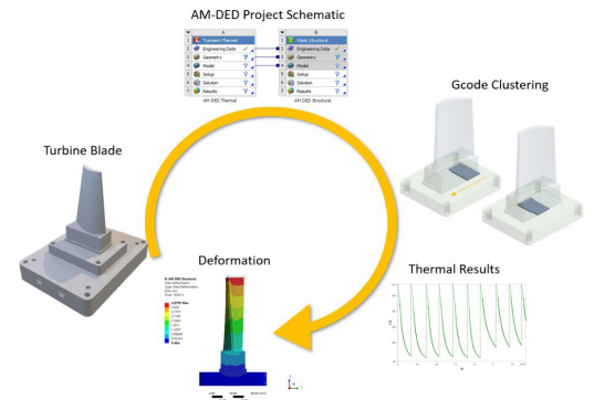
Figure 2. Description of the additive workflow.
