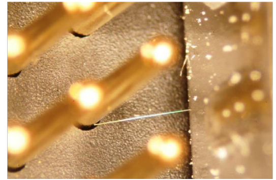
Figure 12. Tin whisker shorting between the bright tin shell and the pin (courtesy of Emerson)
