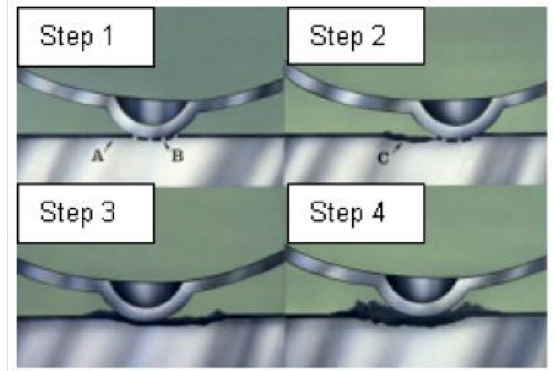
Figure 8. The fretting process for tin-plated contact 3
