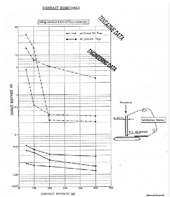
Figure 10. Contact resistance vs. contact normal force for nickel and stainless steel (battery contact normal force was 100-200 grams)
