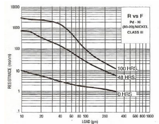
Figure 6. Contact resistance vs. normal force after exposure to mixed flowing gas
