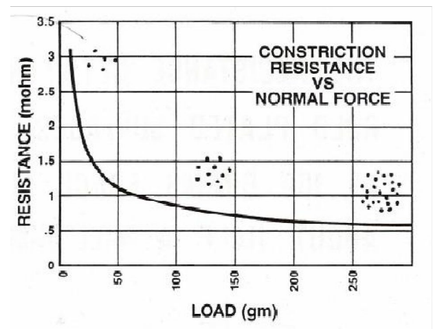
Figure 5. Constriction resistance vs. normal force for a gold-to-gold connection (the small dots represent number of asperities)
