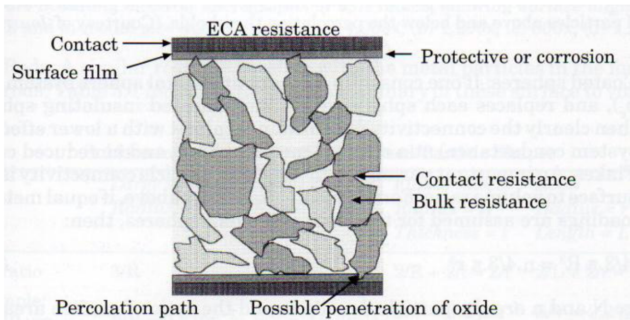
Figure 2. Electrical resistance elements in ICA.
