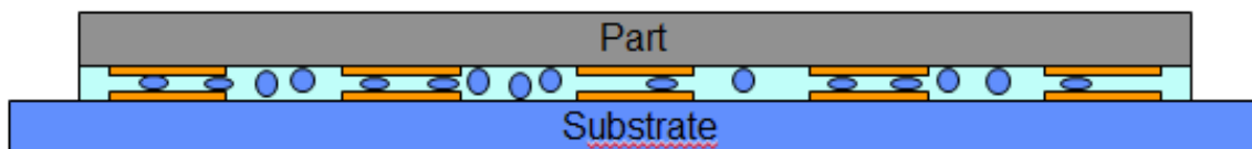
Figure 1: Schematic of ACA interconnection with deformable particles.
