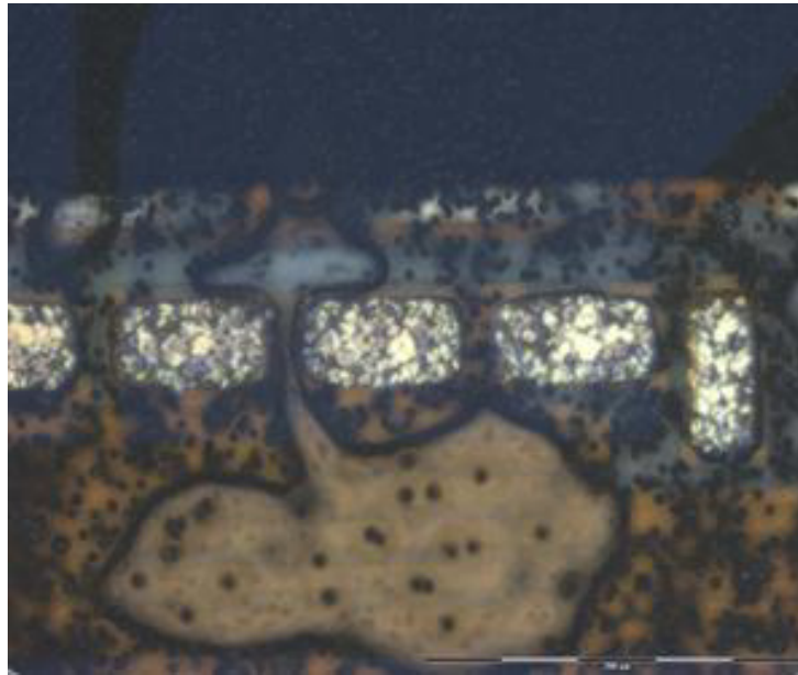
Figure 4: Large air bubble in a chip-on-glass anisotropic conductive film (ACF) interconnection.
