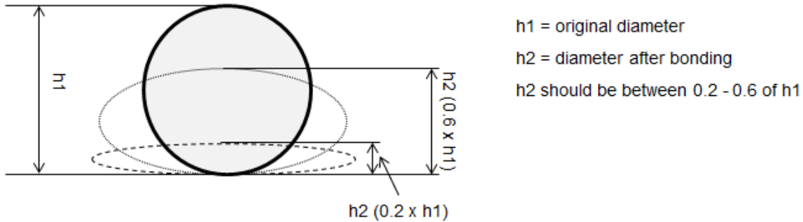
Figure 3: Recommended degree of compression for a conductive particle to ensure compliance
