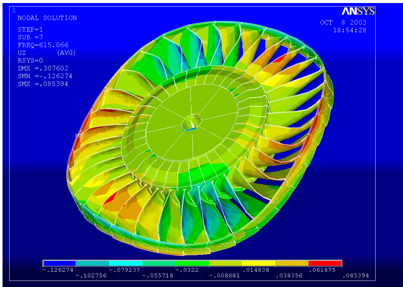
Figure 5. 7 th mode shape of bladed wheel
