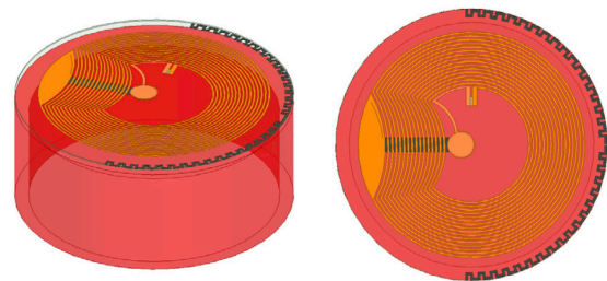
Using Ansys HFSS, a close-proximity wireless power system prototype was designed by maximizing the near-field coupling between the transmitter and receiver antennas.
