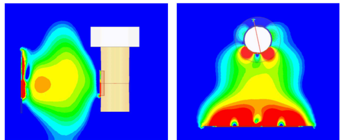
Ansys HFSS was used to design a meandered dipole antenna around an existing RFID tag in a bottle cap.
