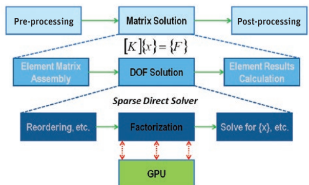
▲ Flowchart for sparse direct solver and GPU acceleration. The computation is offloaded to the GPU during matrix factorization for the sparse direct solver.
