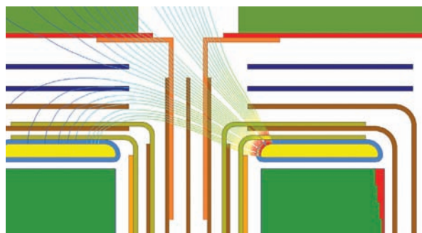
Electric field distribution between two adjacent high-voltage windings
