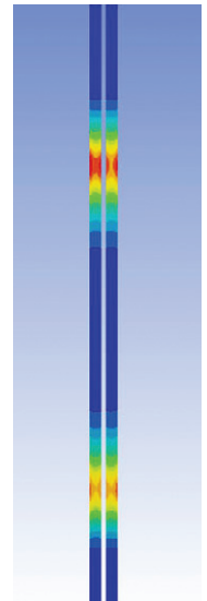
Temperature distribution in coupled ANSYS Mechanical model
