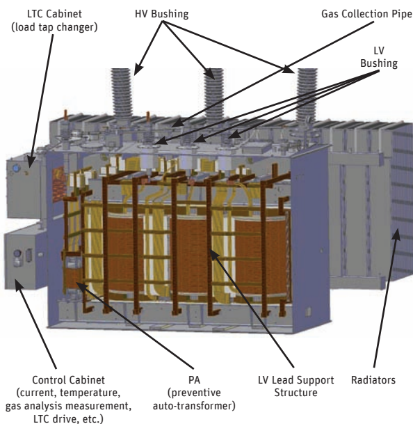
Diagram of a low-voltage power transformer
