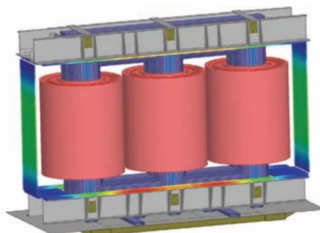
Magnetic flux density distribution in magnetic shunts
