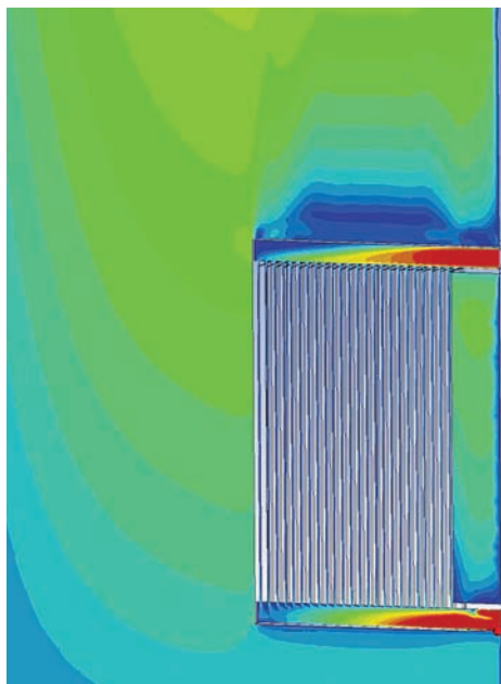
ANSYS Fluent simulation shows velocity contours of oil in radiator fins and air flow around radiator.
