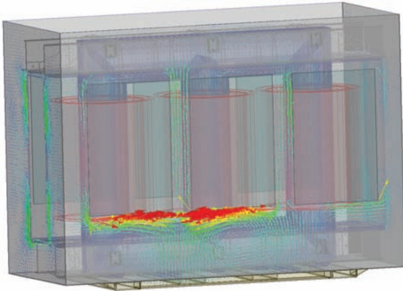
Eddy currents induced by stray fields in tank walls
