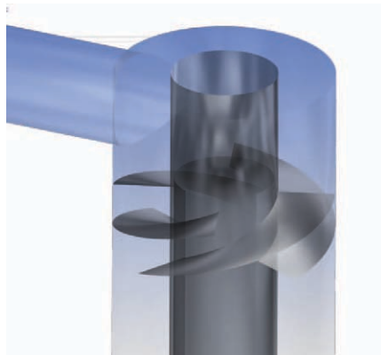
Swirl element fitted in the cyclone
