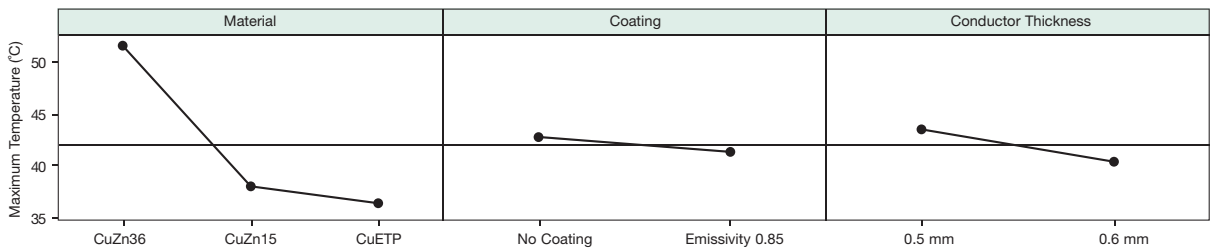
Results from the design of experiments for material, dimensions and radiation coating optimization
