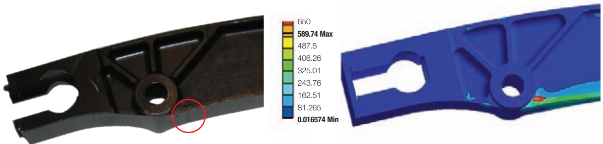
Brake pedal crack with simulation of equivalent stresses
