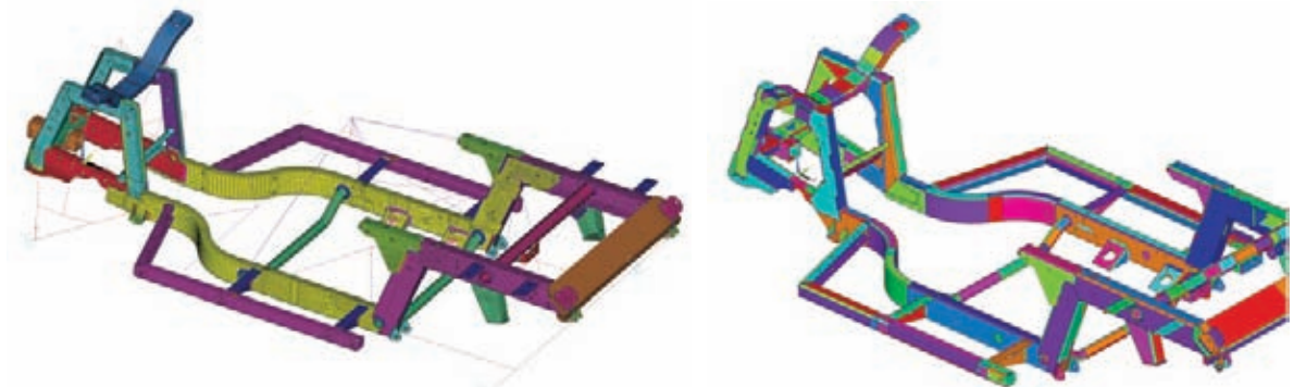
The geometry of the original frame for the utility vehicle (left) and the geometry of the redesigned frame showing welds (right)
