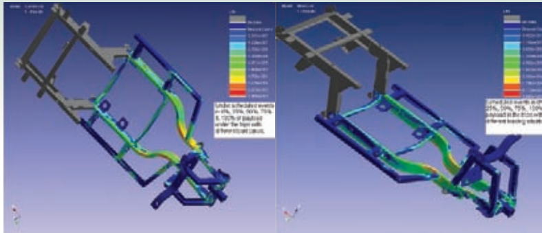
DesignLife (from HBM-nCode) simulation shows the frame life for scheduled events with different payloads for the original frame (left) and the new frame (right)
