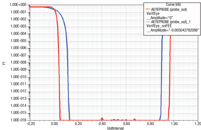
Bathtub curve of feed forward equalization performance generated with the VerifEye tool
