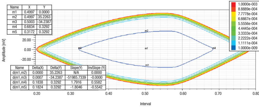
Eye contour plot generated with the VerifEye tool
