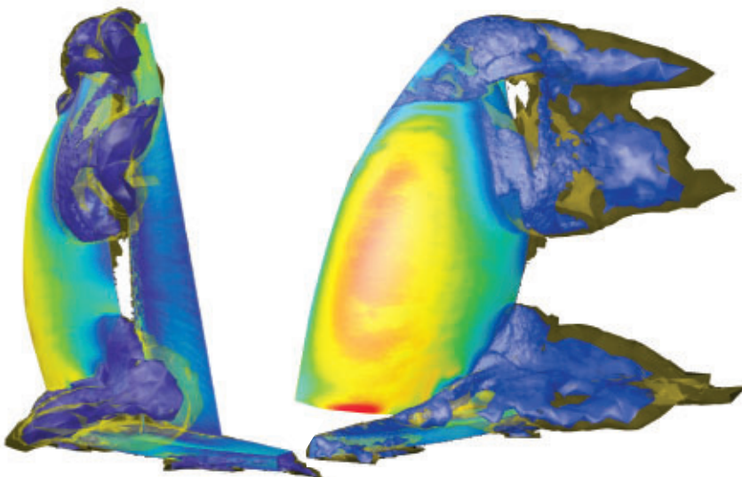
Two leeward (downwind) views, from behind (left) and front (right) showing the air flow velocity over the yacht. The low-velocity regions in blue show vortices from the asymmetric spinnaker and the hull.
