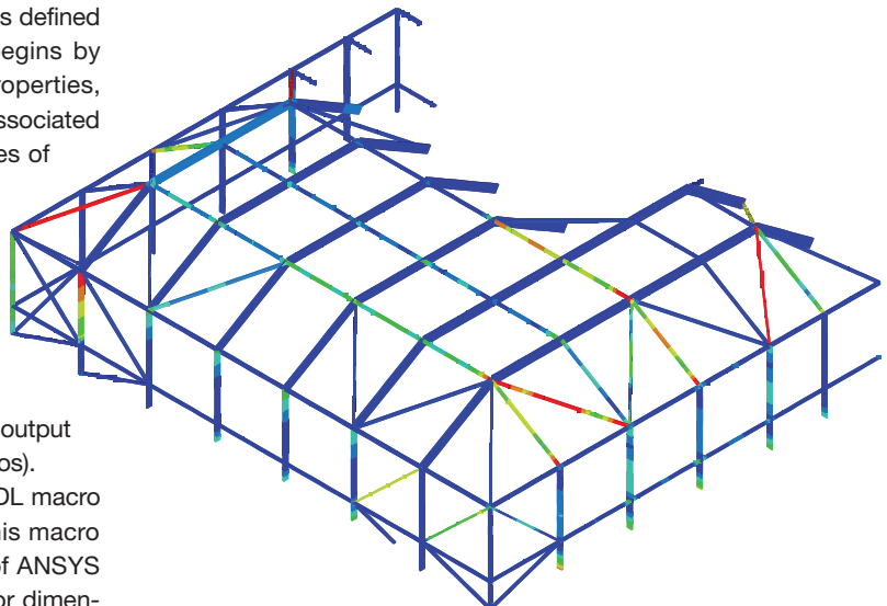
Color contour plots of interaction ratios show locations' potential wind-force failure in red.
