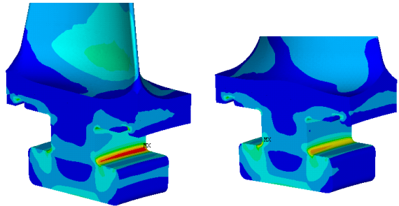
Von Mises stress of modified blade root and neck were significantly lower compared to the initial design in the elastic domain.
