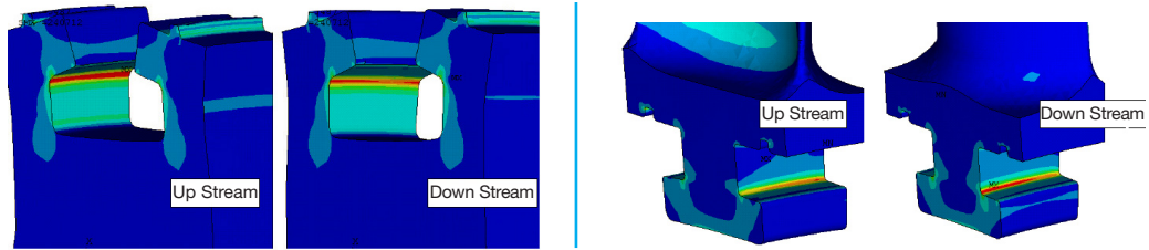
Von Mises stress of unmodified design in elastic domain at 6,000 rpm. Peak stress of 1,904 Mpa is indicated at blade root (left) and 250 Mpa average stress at blade neck (right). Peak stress of 1,660 Mpa is seen at the slot.
