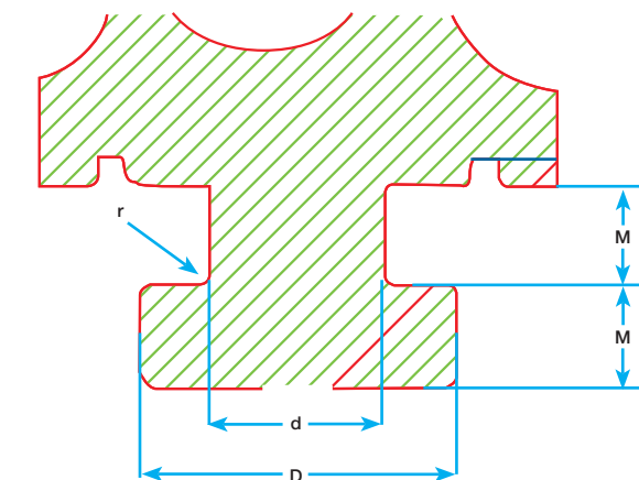
Key blade root dimensions to be modified using ANSYS APDL were root radius r , blade neck d , land height M , and land width D .
