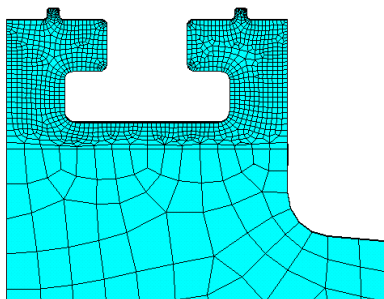
Model of the disk slot ready for analysis
