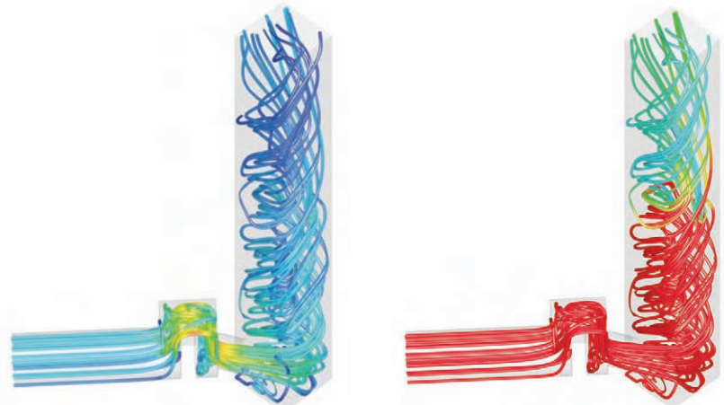
Using fluid dynamics simulation, engineers studied swirling flow and uneven velocity in a gas conditioning system. Design change iterations optimized the design for much more uniform flow velocity (left) and lowered the temperature variations in the stack to within a nominal range (right).
