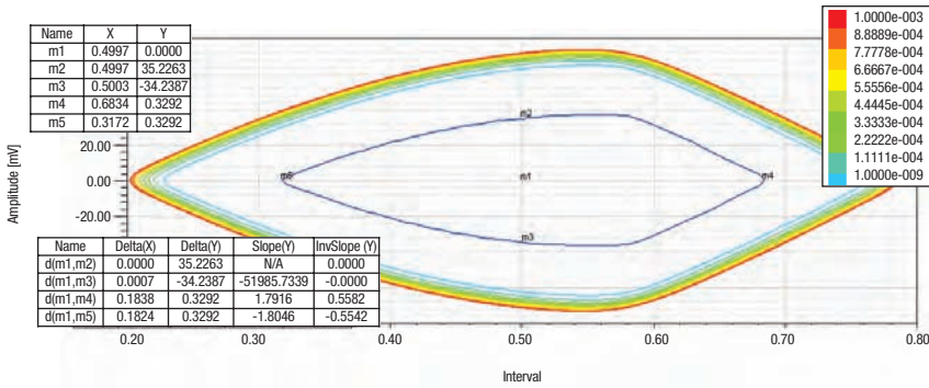
Eye contour plot generated with the VerifEye tool
