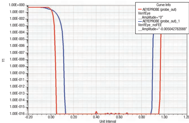
Bathtub curve of feed forward equalization performance generated with the VerifEye tool
