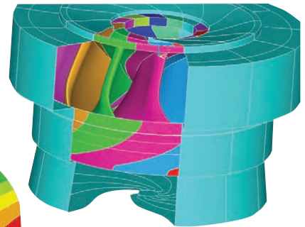
ANSYS model of a hydraulic turbine (top) and FLUID30-based pressure field (bottom) Images courtesy Voith Hydro.
