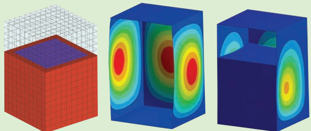
The influence of the additional mass of water on vibration modes of a rectangular tank is shown in models of a partially filled tank (left), an uncoupled structural dry mode of the empty tank at 33 Hz (middle), and a coupled wet mode at 10 Hz taking into account FSI using ANSYS SHELL181/FLUID30 coupling (right).
