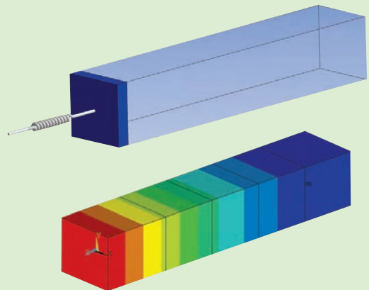
Gases add stiffness to the containing structure, as in the piston shown here supported by a spring and an attached air enclosure (top) with an uncoupled dry mode at 40 Hz and a coupled wet mode at 80 Hz. Pressure mode of the cavity (bottom) was found using ANSYS FLUID30 elements to analyze the system.
