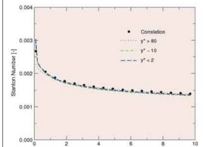
Figure 4: Grid sensitivity for wall heat transfer predictions.
