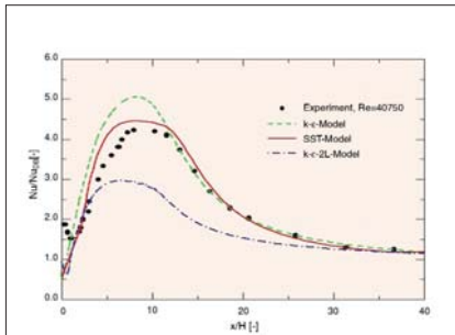
Figure 3: Non-dimensional wall heat transfer coefficient for an axisymmetric sudden pipe expansion [3]
