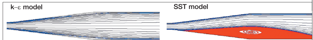
Figures 1 and 2: Streamlines for plane diffuser flow for both models. The SST model predicts the separation zone in close agreement with data, whereas the k-\epsilon model fails to capture the physics of this flow entirely.
