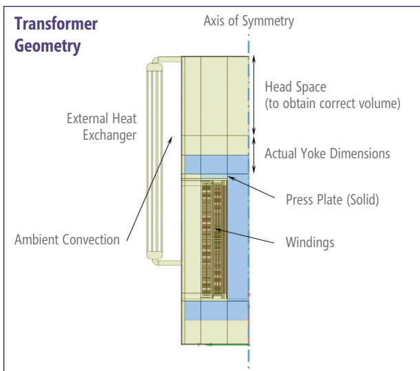
Figure 1: SpaceClaim model of a simplified Waukesha Electric medium-sized electrical power transformer. The geometry in blue represents the yoke and core. Low and high-voltage windings surround the coil. An external heat exchanger is used to dissipate electrical power losses to the environment.
