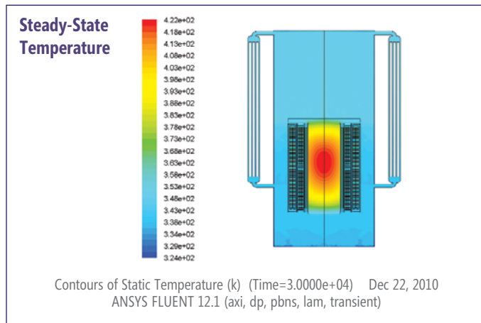
Figure 3: Contours of the steady-state temperature distribution inside the transformer. Simulation was performed using ANSYS FLUENT 12.
