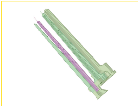
When conducting a flow analysis, the plunger, cooling tube parts, and air volume are created using ANSYS SpaceClaim.
